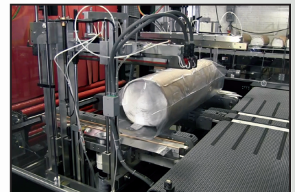
108-100 Side Seal Assembly for a Totally Enclosed Package
